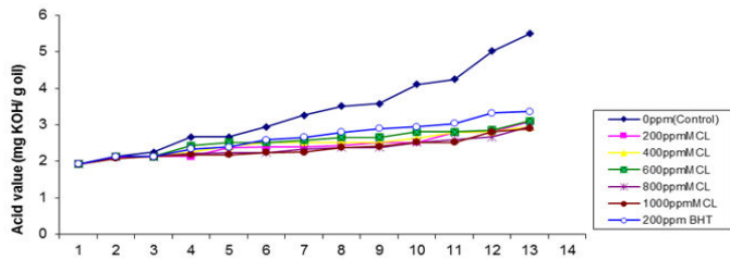
Figure 2: Acid value of refined palm kernel oil stored with Methanol Chaya Leaf (MCL) extract and BHT for twelve months.
