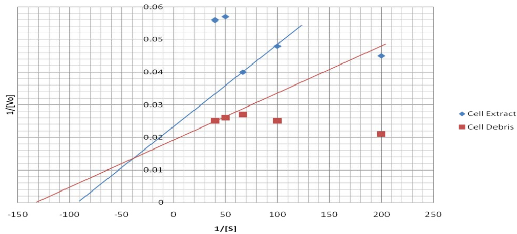
Figure 5) Lineweaver-Burk plots of NDMA formation in cell extract and cell debris of Bacillus cereus at a fixed DMA concentration and varying \text{NaNO}_2 concentrations
