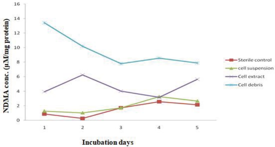
Figure 3) Concentrations of NDMA formed by Bacillus cereus incubated with DMA and sodium nitrate
