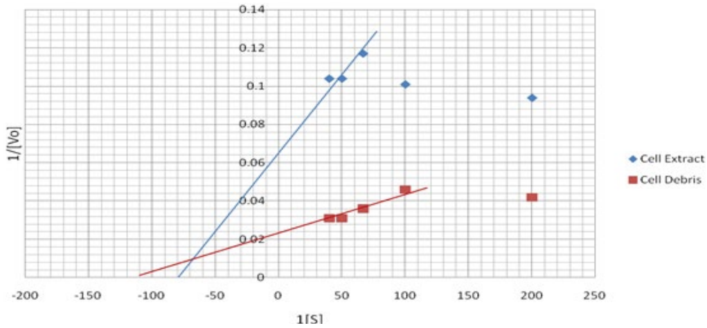
Figure 4) Lineweaver-Burk plots of NDMA formation in cell extract and cell debris of Bacillus cereus at a fixed \text{NaNO}_2 concentration and varying DMA concentrations
